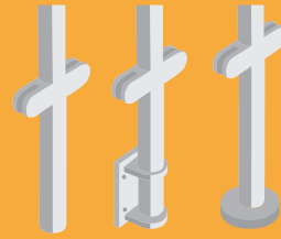
Surface, Fascia and Embed mount posts
