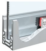
PanelGrip® Standard
